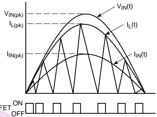
Figure 24. Inductor Waveform During CRM Operation
